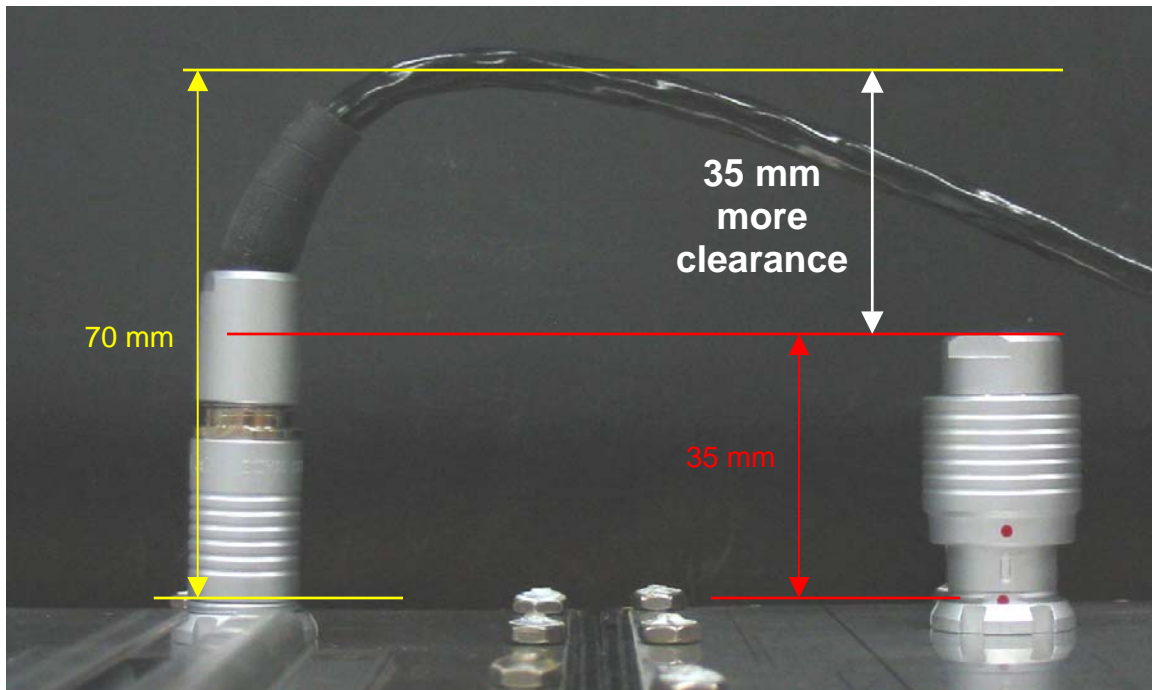
Comparison of Standard and Right Angle Connector Plugged into RMC-1 Receiver
